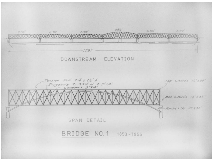
Schematics
